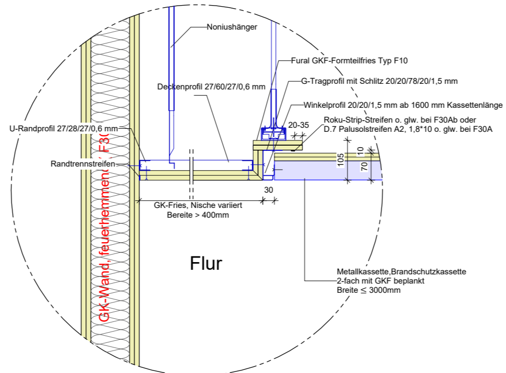
Detail F
