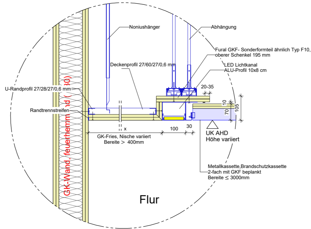
Detail E
